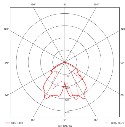
GAFIM 250 MIH
