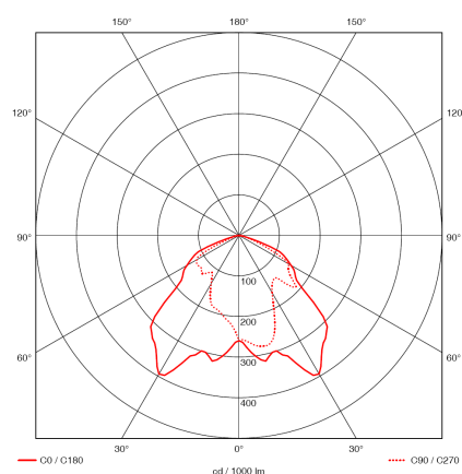
GAFIM 400 MIH
