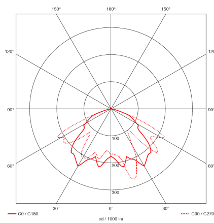
GAFIM 250 MIH
